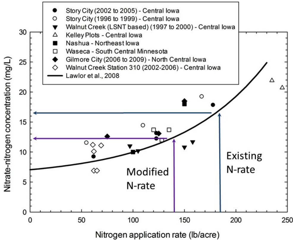
Figure 4. Overall nitrogen application rate effect on nitrate-N concentration in tile drainage.
