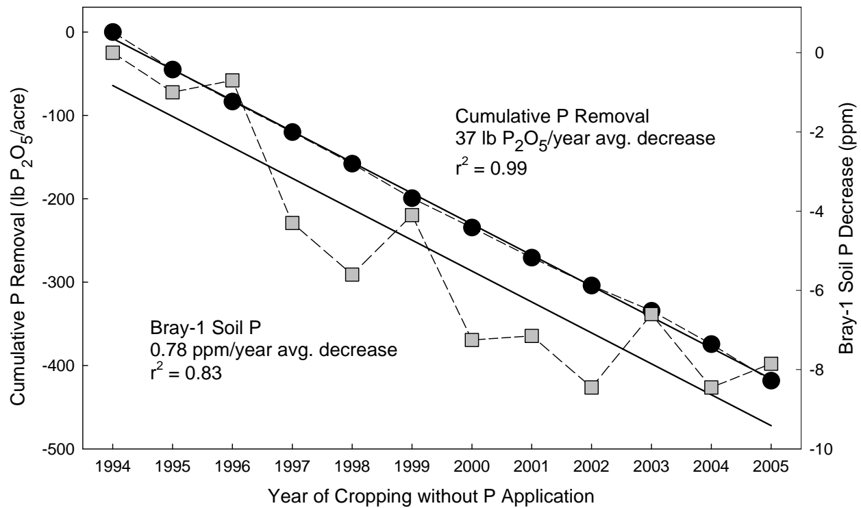
Fig. 4. Trends over time of P removal for corn-soybean rotations and soil-test P for plots that received no P fertilizer. Averages across five Iowa locations. Adapted from Mallarino and Prater, 2005.
