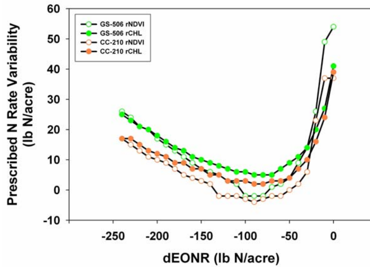
Fig. 3. Sensor prescribed N rate variability across deficit differential economic optimum N rates (dEONR) for relative canopy indices from the GreenSeeker 506 (GS-506) and Crop Circle ACS-210 (CC-210) active sensors.
