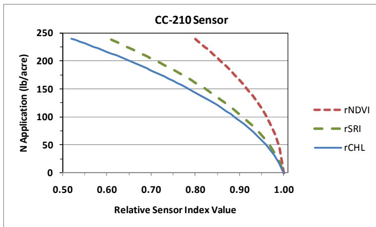
Fig. 2. Nitrogen rate application prescriptions derived from the calibration models for the relative canopy indices from the GreenSeeker 505 (GS-505), GreenSeeker 506 (GS-506), and Crop Circle ACS-210 (CC-210) active sensors.
