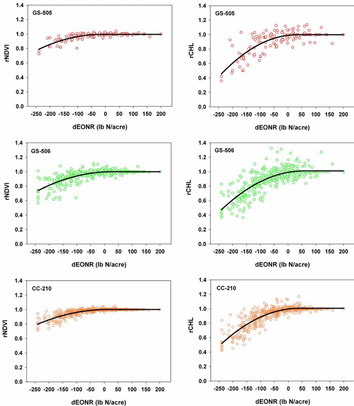
Fig. 1. Relative canopy index values and regression models as related to the differential from the economic optimum N rate (dEONR) for the GreenSeeker 505 (GS-505), GreenSeeker 506 (GS-506), and Crop Circle ACS-210 (CC-210) active sensors.
