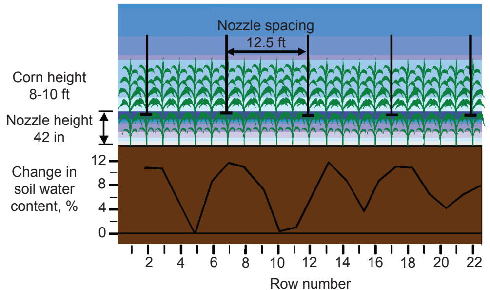
Figure 13. Change in soil water content resulting from a single sprinkler application event using low pressure spray nozzles positioned 3.5 feet above the soil surface and a nozzle spacing of 12.5 feet between nozzles.
